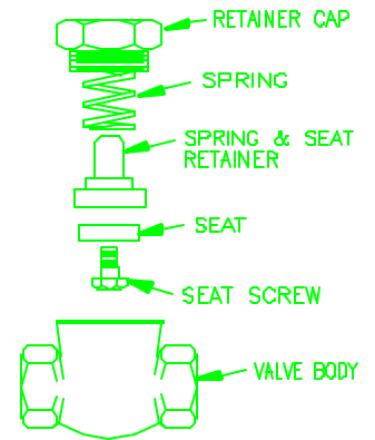
HORIZONTAL SPRING LOAD CHECK VALVE 25606
