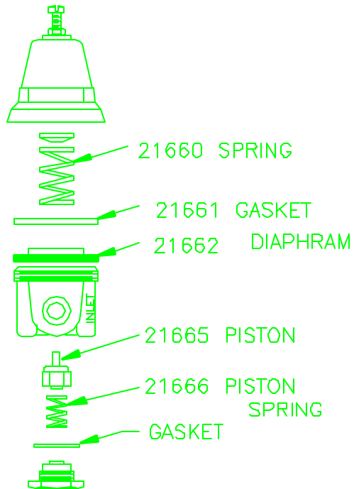
1/4"REGULATOR 16048
