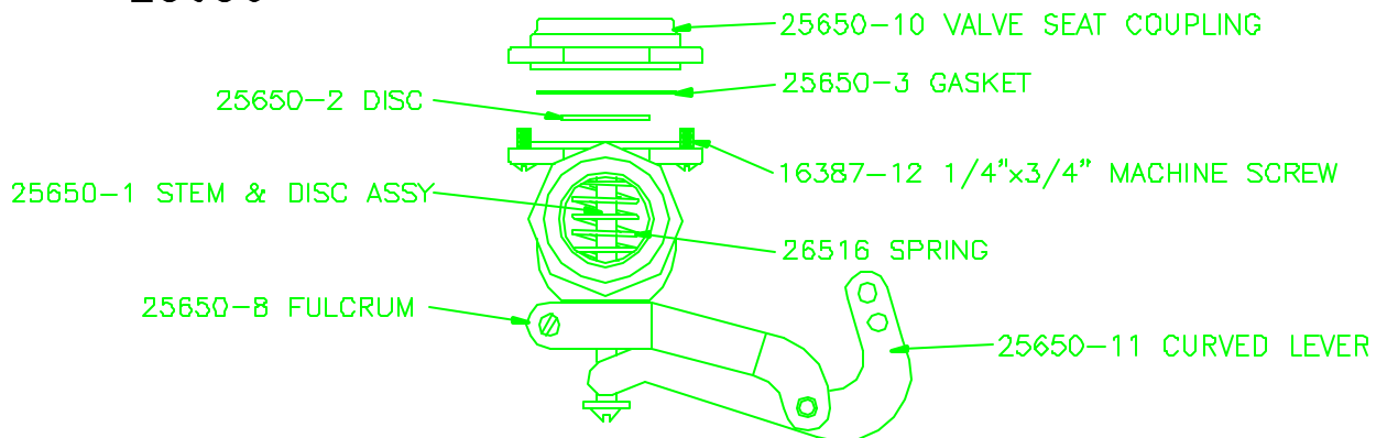
VACUUM VALVE 25650
