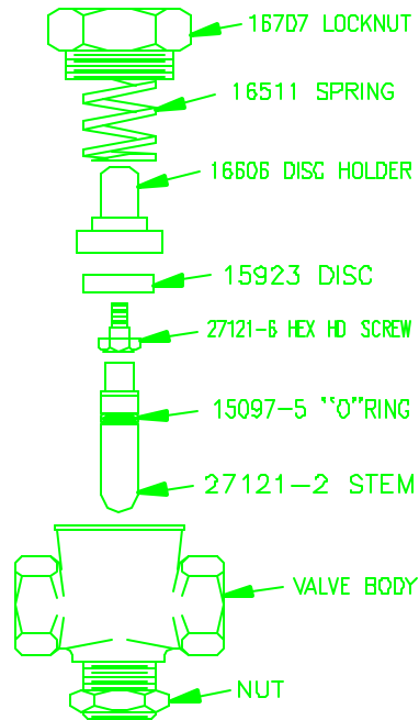
1/4" AIR WHISTLE VALVE 15100
